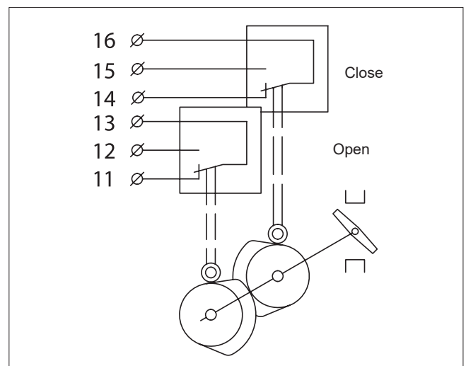
Fig. 32 Limit switch adjustment, 2 switches
