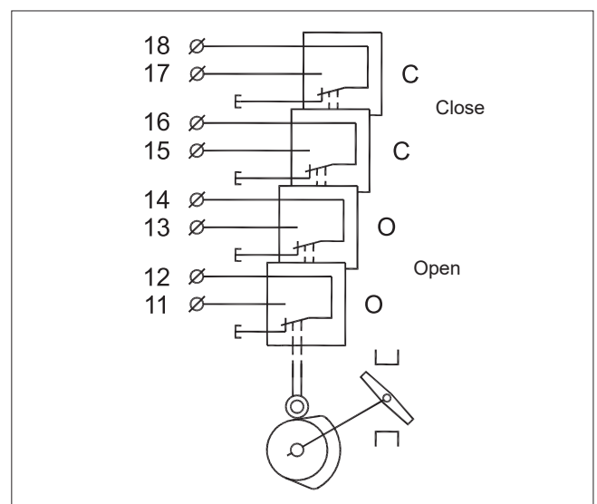
Fig. 33 Limit switch adjustment, 4 switches
