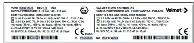
Fig. 2 Examples of identification plate
